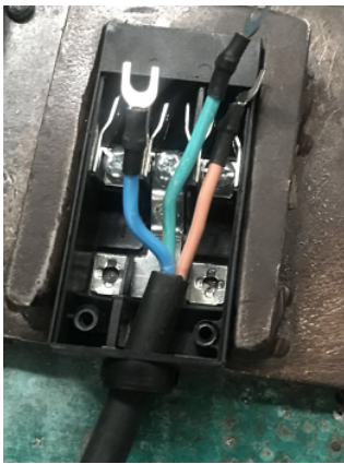
Put the supply cable into the terminal board
