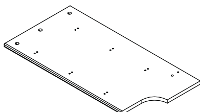
13 Partition x1 (71.4x36.1x1.6cm) No. 4301-1607142-40
