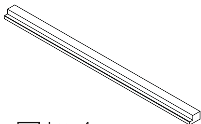
4 Leg x4 (71.4x4.0x2.6cm) No. 12-02607141-20
