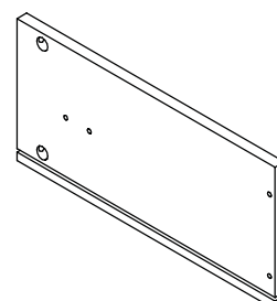
9 Drawer side Left x6 (35x16.7x1.3cm) No. 15-01303504
