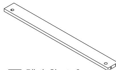
6 Plinth Short x2 (68.3x6.5x1.5cm) No. 12-01506831
