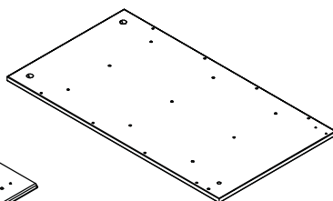
2 Side panel Right x1 (65.4x36.1x1.2cm) No. 4301-1206541-40
