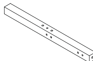
11 Leg Left x2 (60,7x4,3x4,3cm) No. 12-04306072-40
