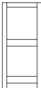
4 Short side panel x2 (53.5×22cm)
