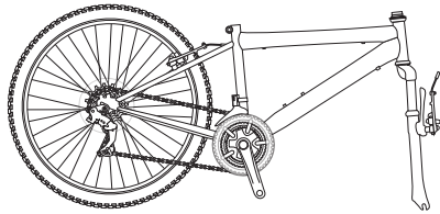
Frame Assembly
