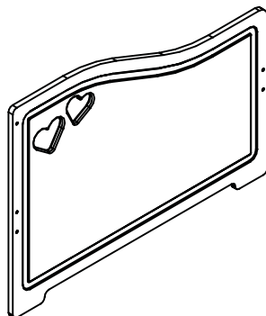
2 End panel Left x1 (95,4x68,0x1,6cm) No. 4301-1609542-40
