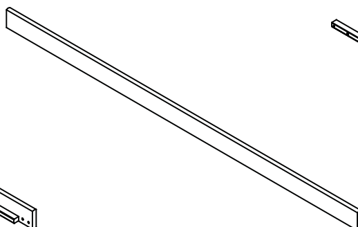
8 Back rail x1 (190,0x8,9x2,0cm) No. 12-02019002-40
