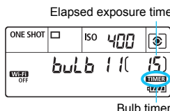
Bulb timer
