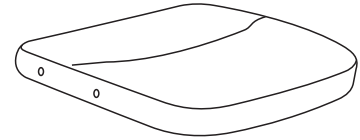
3 Seat (480x485x65mm)
