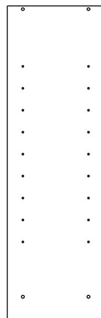
1 Right side (915x290mm)
