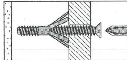
No.3 "Cavity Fixing" wall plug
