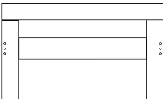
2 Footboard (61.8 x 97.1cm)
