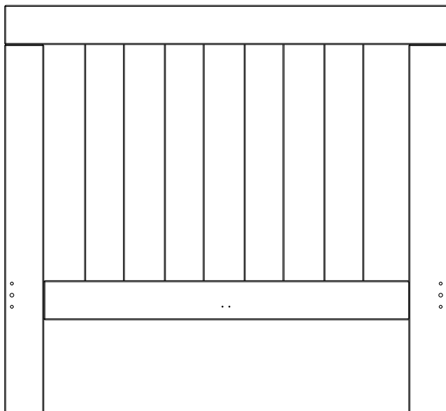
1 Headboard (112.8 x 128.1cm)
