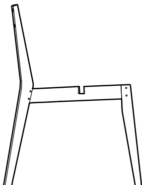
1 Chair frame x 2 (75.6 x 57.5cm)
