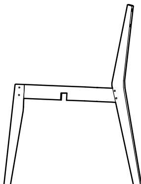
2 Chair frame x 2 (75.6 x 57.5cm)
