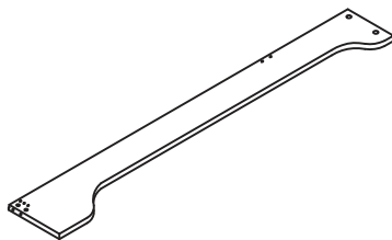
2 Upper right side panel x 1 (132(w)cm x 19.5(d)cm)
