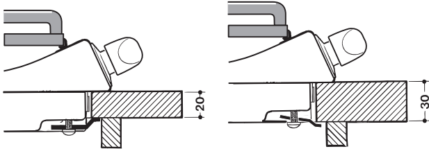
Hooking position for top H=20mm
