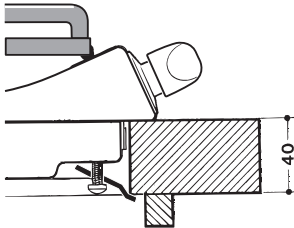
Hooking position for top H=40mm
