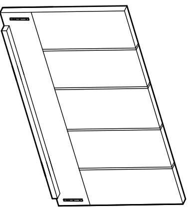
1 Headboard (143x92cm)
