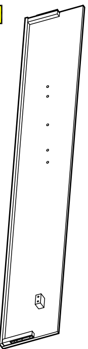
3 Side rail x 1 (194x33cm)
