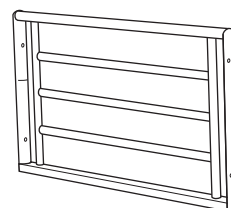
6 Upper side safety rail x 2 (91 x 36 x 4cm)
