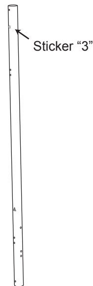
3 Front right-hand end post (Ø5 x 165cm)
