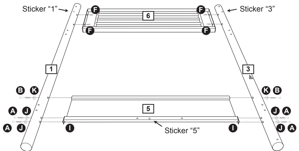
RIGHT-HAND END PANEL
