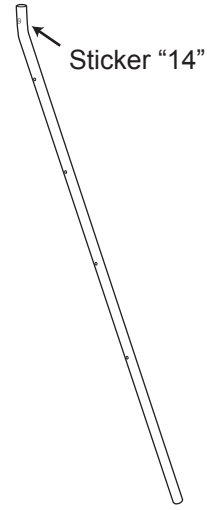
14 Right ladder side rail (150 x Ø2.5cm)
