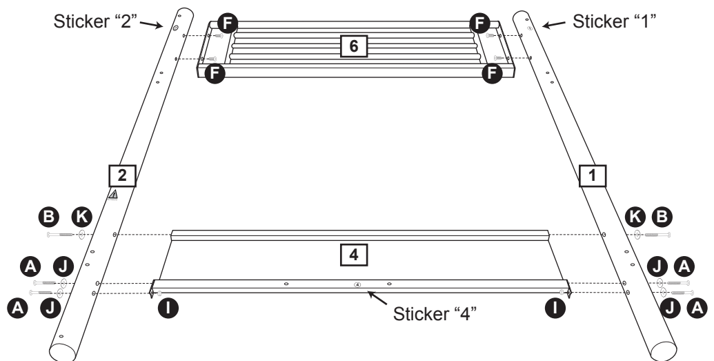
LEFT-HAND END PANEL
