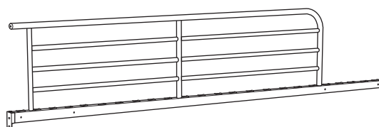
8 Upper front safety rail (190.5 x 41.5 x 2.5cm)
