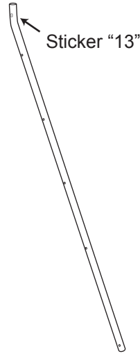
13 Left ladder side rail (150 x Ø2.5cm)
