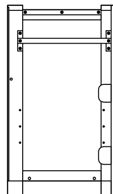
3 Side panel (Left) (75 x 43 cm)
