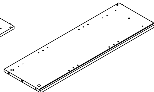
3 Right side x1 (82cm x 26.2cm)
