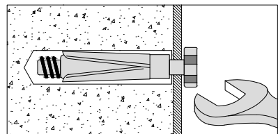
No.4 "Shield Anchor" wall plug - heavy loads
