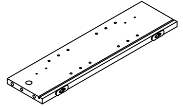
3 Left side x1 (45.4cm x 11.9cm)
