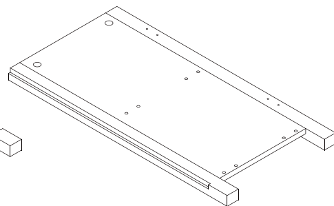
3 Right Side Panel x 1 (58.5(w)cmx28.4(d)cm)
