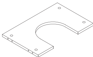
4 Bottom panel x 1 (43(w)cmx28(d)cm)
