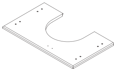
1 Top panel x 1 (51.5(w)cmx30(d)cm)
