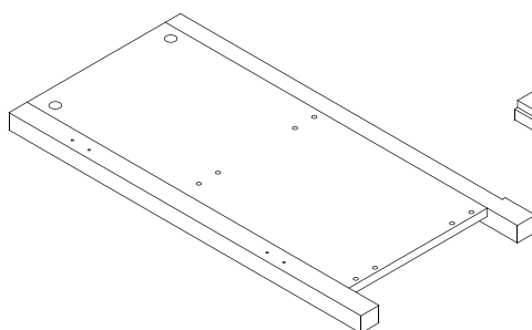
2 Left Side Panel x 1 (58.5(w)cmx28.4(d)cm)
