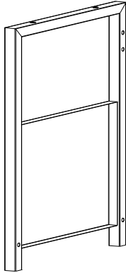
13 Cart left side panel assembly x 1
