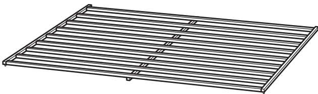
3 Slat x 2 (137 x 90.5 x 3.2cm)
