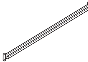
4 Siderail x 2 (190 x 12 x 4.5cm)
