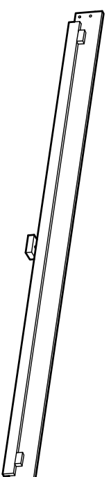
4 Side rail x 1 (192x13.5cm)
