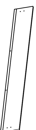
8 Front board x 1 (191x20.5cm)
