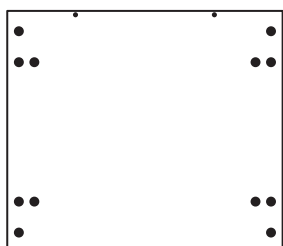
4 Top/Base (DPF078B) (569 x 494mm) x 2
