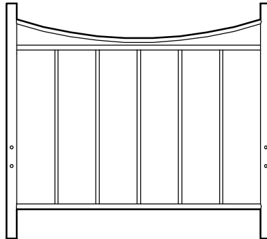
2 Footboard frame (95.7 x 87.5cm)
