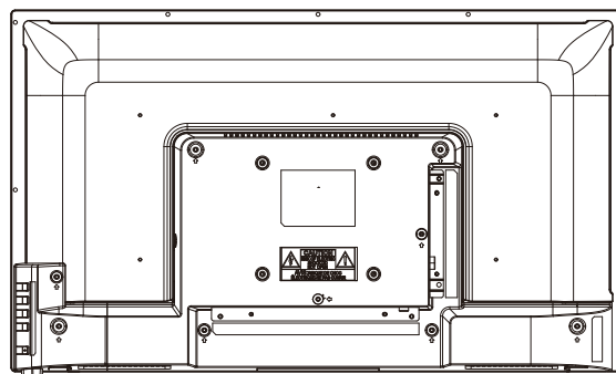
100 x 100mm VESA mount
