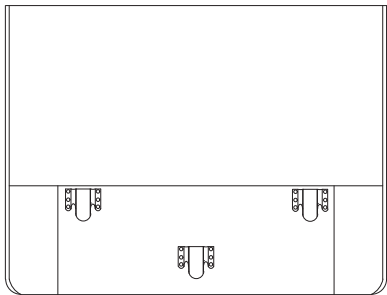
7 Side arm ( Right ) 910 x 540 x 175mm
