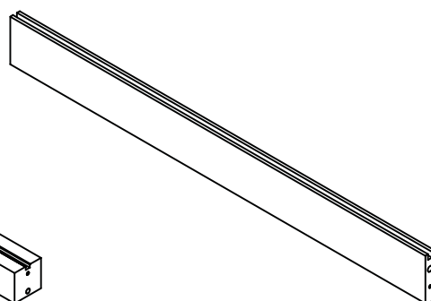
8 Endrail x2 (86,5x8,9x2,0cm) No. 12-020086510-20
