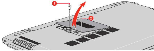
Figure 4-6 Removing the memory module cover
