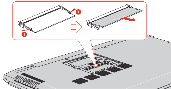
Figure 4-9 Removing the memory module
