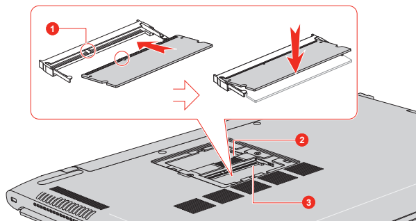
Figure 4-7 Seating the memory module
