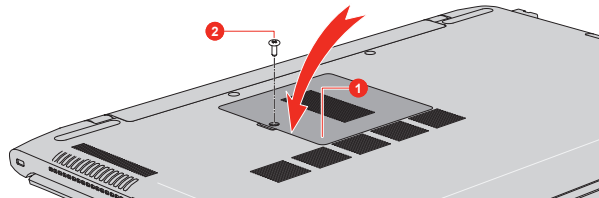
Figure 4-8 Seating the memory module cover
