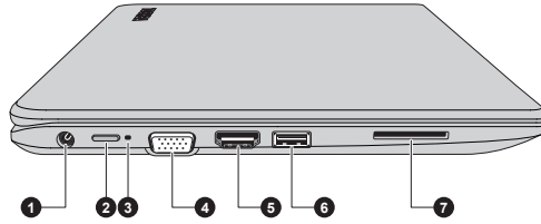
Figure 3-2 The left side of the computer (CL10-C/L10-C)
