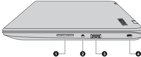
Figure 3-10 The right side of the computer (CL10W-C/L10W-C)
