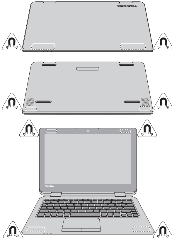
Figure 3-14 Magnets location (CL10W-C/L10W-C)
