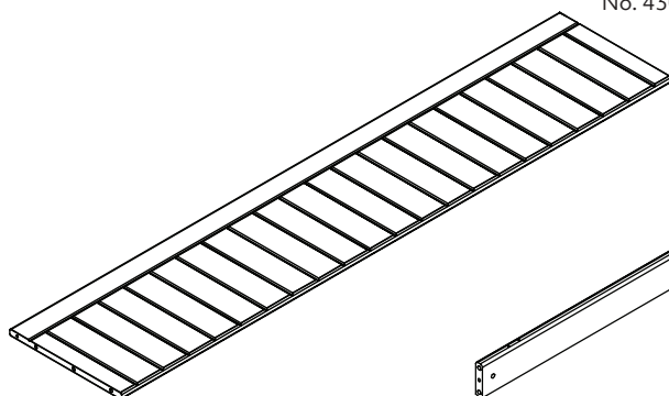
7 Back panel x1 (1868x380x19mm) No. 4301-1918681-40 White No. 4301-1918681-65 Grey
