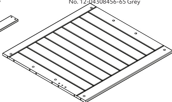
5 End panel left x1 (877x835x19mm) No. 4301-1908773-40 White No. 4301-1908773-65 Grey
