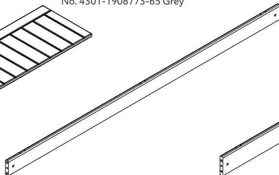
8 Bedside x1 (1868x89x20mm) No. 12-02018684-20 White No. 12-02018684-65 Grey
