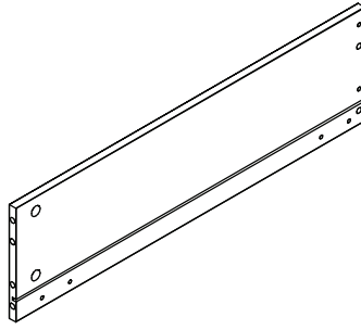
14 Drawer side left x1 (600x170x12mm) No. 4301-1206002-40 White No. 4301-1206002-65 Grey
