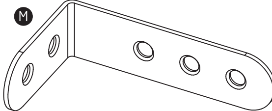
M Angle 70x40,5x20mm x2 No. 4008-022
