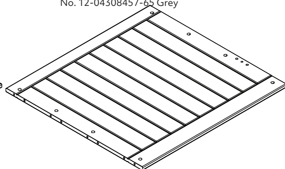
6 End panel right x1 (877x835x19mm) No. 4301-1908772-40 White No. 4301-1908772-65 Grey
