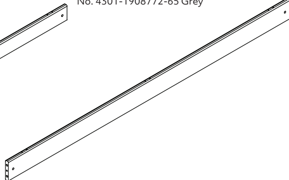
9 Bedside x1 (1892x115x20mm) No. 12-02018921
