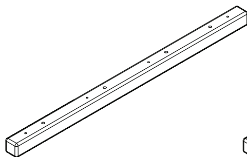
1 Leg front x2 (845x43x43mm) No. 12-04308458-20 White No. 12-04308458-65 Grey
