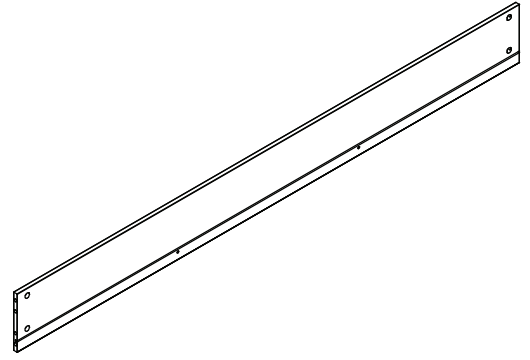
15 Drawer back x1 (1690x170x12mm) No. 4301-1216901-40 White No. 4301-1216901-65 Grey
