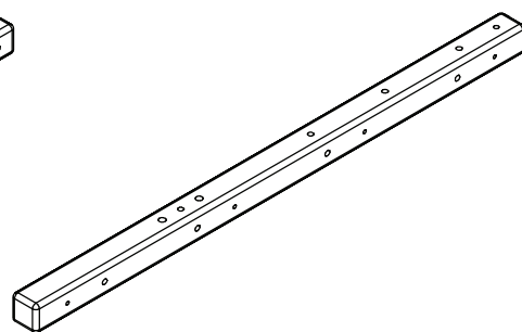
3 Leg back right x1 (845x43x43mm) No. 12-04308457-20 White No. 12-04308457-65 Grey
