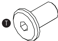
T Sleeve nut Ø8/M6x15mm x4 No. 3923-06015
