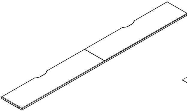
16 Drawer front x1 (1860x230x19mm) No. 4301-1918601-40 White No. 4301-1918601-65 Grey
