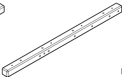
2 Leg back left x1 (845x43x43mm) No. 12-04308456-20 White No. 12-04308456-65 Grey
