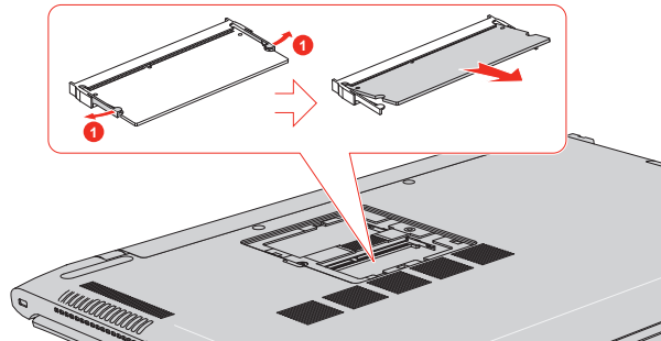
Figure 4-9 Removing the memory module
