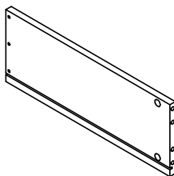
5 Drawer side right x2 (45x17x1.5cm) No. 15-01504501-20
