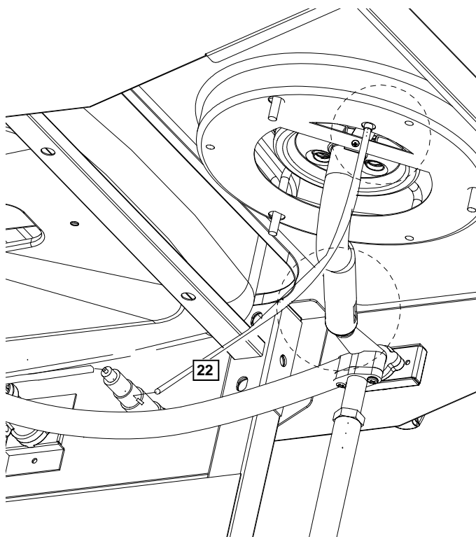
Electrode of Main Burner
