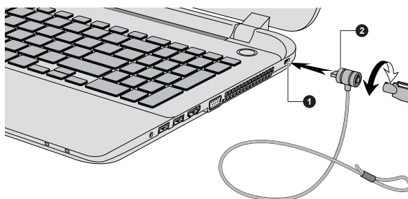
Figure 4-10 Security lock
