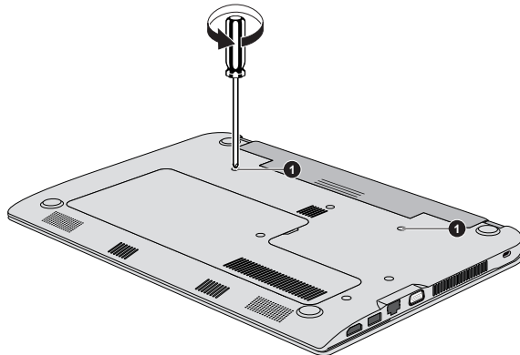
Figure 4-2 Loosening the screws
