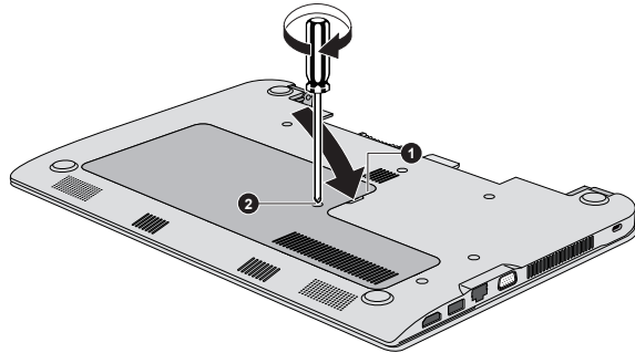
Figure 4-7 Seating the memory module cover
