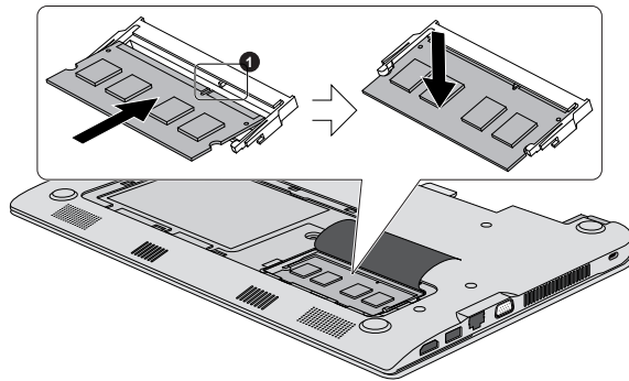
Figure 4-8 Seating the memory module
