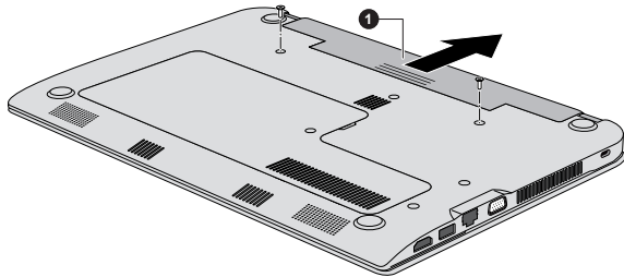
Figure 4-3 Releasing the battery pack
