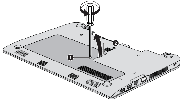
Figure 4-5 Removing the memory module cover
