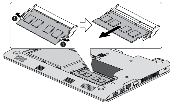
Figure 4-6 Removing the memory module
