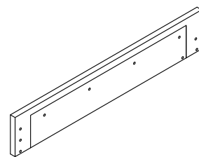
3 Side Rail 01 x2 (955 X 175 mm)
